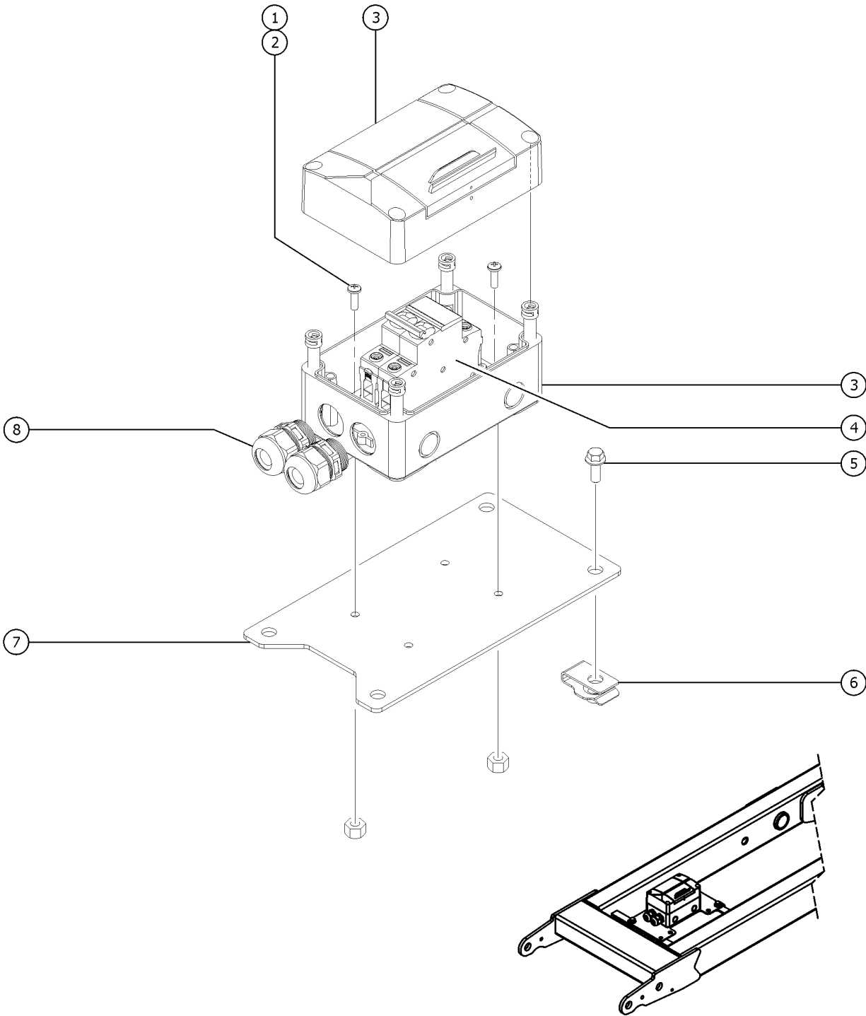
MOUNTING LOCATION ON LINKSTACK
